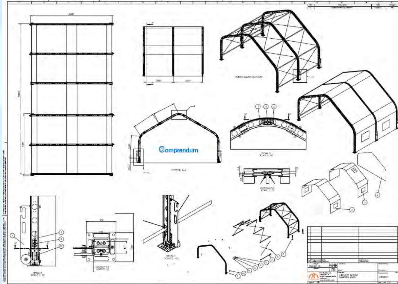
S-Model aluminium beamed tent width 6 meter, lengths 5 – 20 meters
